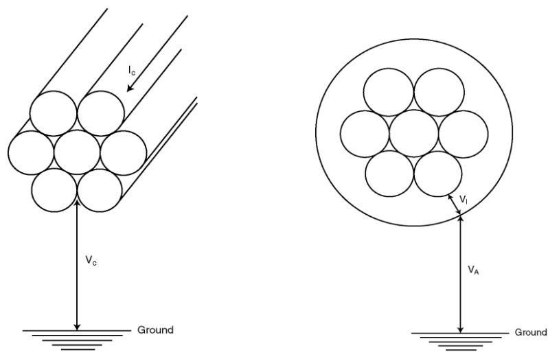
Figure 22 – Location of voltage
