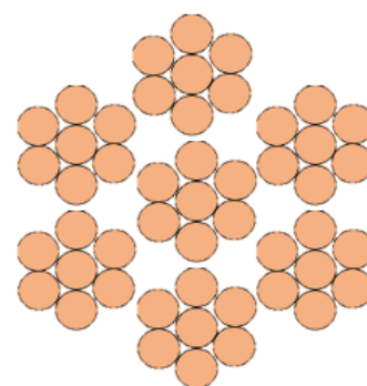
Figure 18 – Rope-lay conductor
